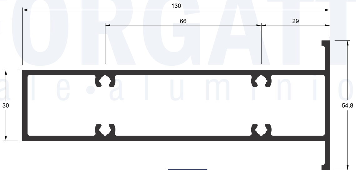
P-278 2,201 kg/m
