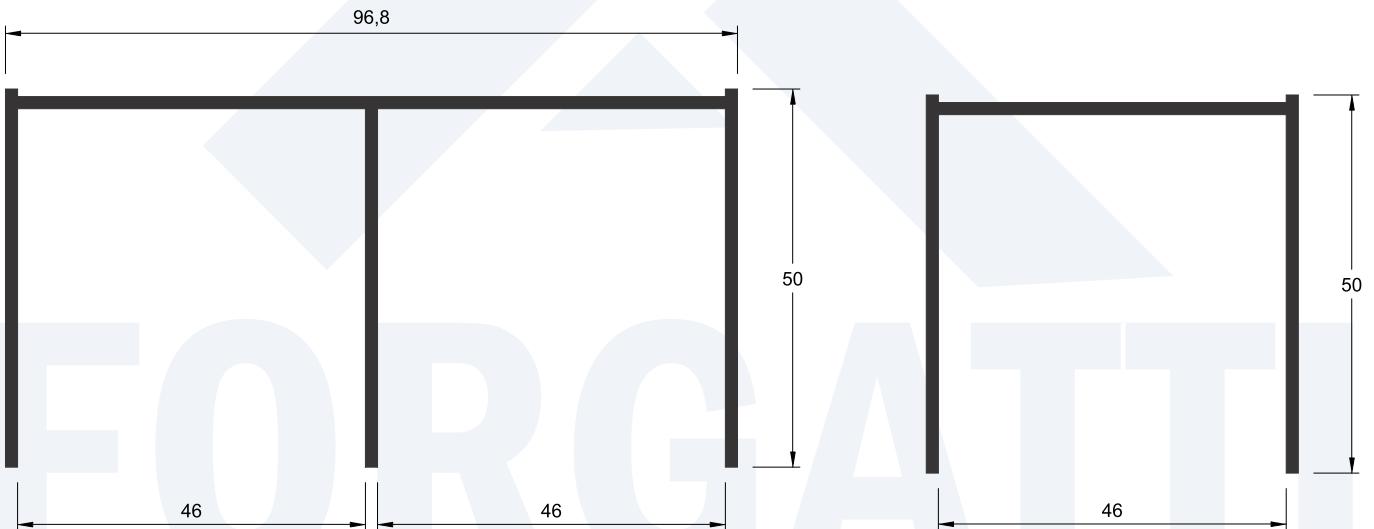
E-363 1,043 kg/m
